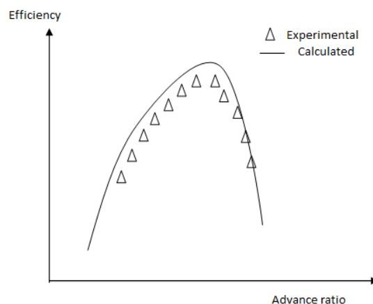
Fig.1 Efficiency drop in different advance ratios[3]
