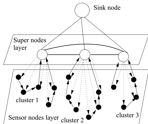
Fig. 1. Layered sensor network
