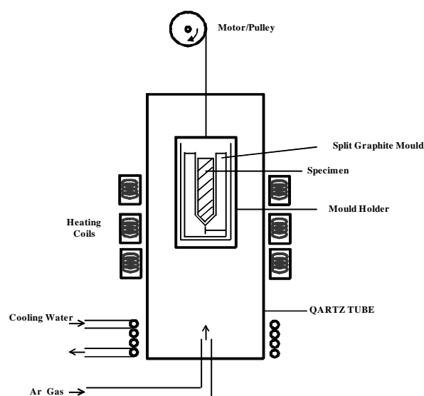
Fig. 1 Schematically illustrated apparatus for single crystal growth
