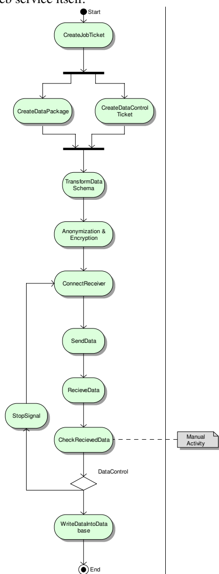
Fig. 2: BPEL activity steps
