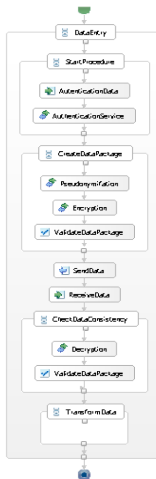
Fig. 3: BPEL-Model for the data entry process
