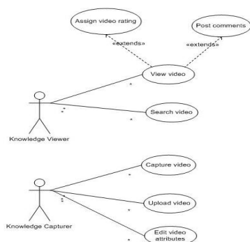
Fig. 1 Use Case Diagram of NMS
