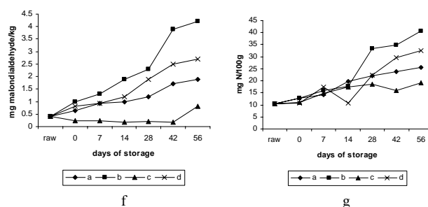
Fig.2. Impact of the processing conditions and storage temperature on the (f) Thiobarbituric acid value and (g) TVB-N values in carp filets processed by sous vide method. Control and 2 °C for storage (a), control and 10 °C (b), sauced and 2 °C (c) and sauced and 10 °C (d). Each point is the mean of three samples taken from three replicate experiments (n= 3x3). Error bars show SD.
