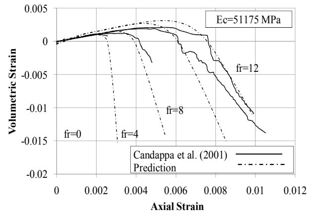
Fig. 10 Comparison of the volumetric strain Vs. axial strain for [12] test results ( f'c=100 MPa) with Proposed Model
