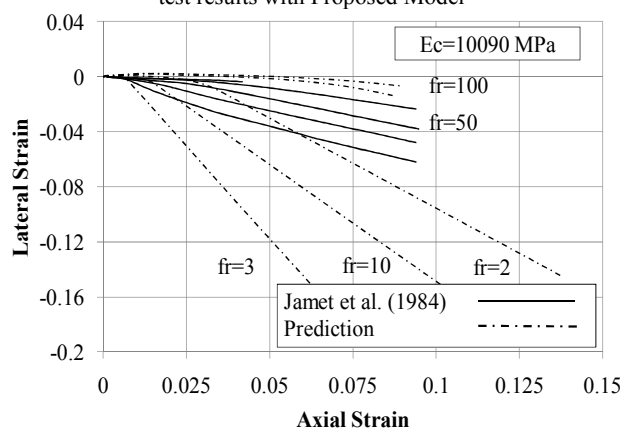
Fig. 12 Comparison of the volumetric strain Vs. axial strain for [13] test results with Proposed Model
