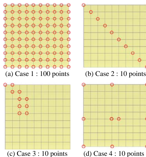
Fig. 7 Arrangements of microphones to evaluate the effect of the location of the sensors
