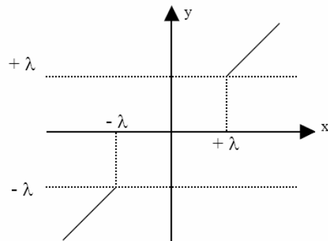
Fig. 5 (b): Hard-Thresholding
