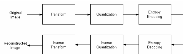
Fig. 1 Generic transform coding for digital images
