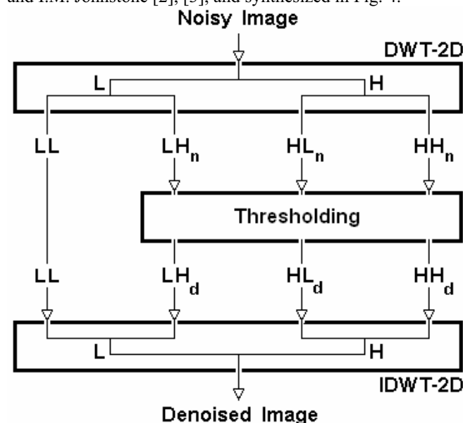
Fig. 4 Thresholding Techniques
