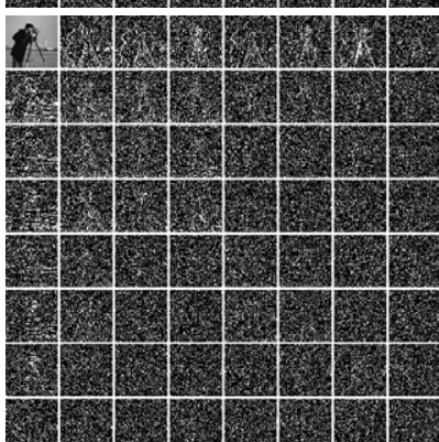
Fig. 17 Comparison of efficiency: (a) sub-blocks set for Morton's scan + KLT, (b) eigenvalues distribution for Morton's scan + KLT, (c) sub-blocks set for row-rafter scan + KLT, (d) eigenvalues distribution for row-rafter scan + KLT, (e) sub-blocks set for Haar + Morton's scan + KLT, (f) eigenvalues distribution for Haar + Morton's scan + KLT, (g) sub-blocks set for Haar + row-rafter scan + KLT, and (h) eigenvalues distribution for Haar + row-rafter scan + KLT
