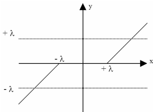
Fig. 5(a) Soft-Thresholding
