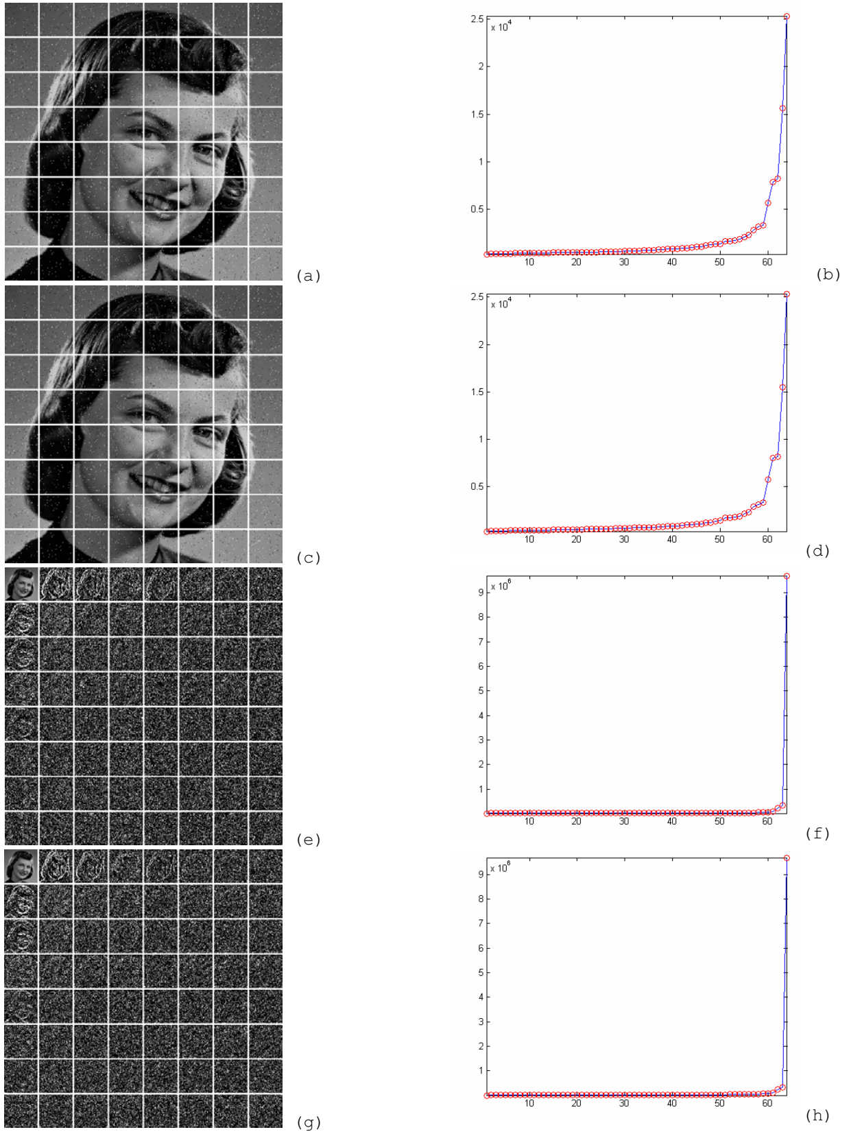
Fig. 21 Comparison of efficiency: (a) sub-blocks set for Morton's scan + KLT, (b) eigenvalues distribution for Morton's scan + KLT, (c) sub-blocks set for row-rafter scan + KLT, (d) eigenvalues distribution for row-rafter scan + KLT, (e) sub-blocks set for Haar + Morton's scan + KLT, (f) eigenvalues distribution for Haar + Morton's scan + KLT, (g) sub-blocks set for Haar + row-rafter scan + KLT, and (h) eigenvalues distribution for Haar + row-rafter scan + KLT
