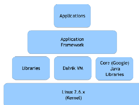
Fig. 2 Hierarchical View of the Android Framework [11]
