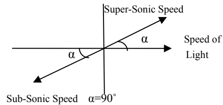
Fig. 4 Random Exiting Process
