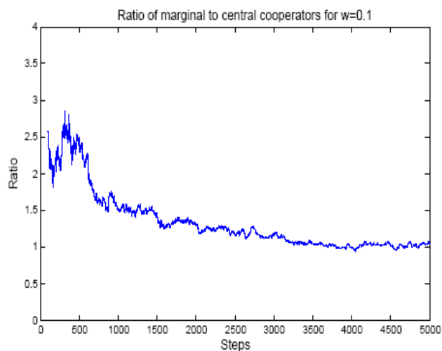
Fig. 4 Ratio of cooperators in marginal nodes to central nodes during evolution. There are more cooperators in marginal nodes than central nodes.
