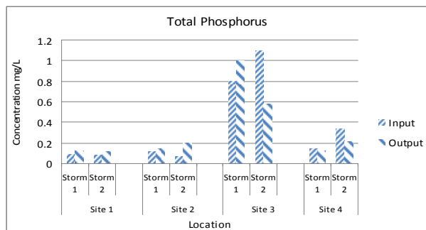
Fig. 7 Total Phosphorus concentrations at each site
