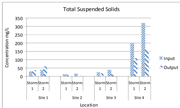
Fig. 5 Total Suspended Solids concentrations at each site
