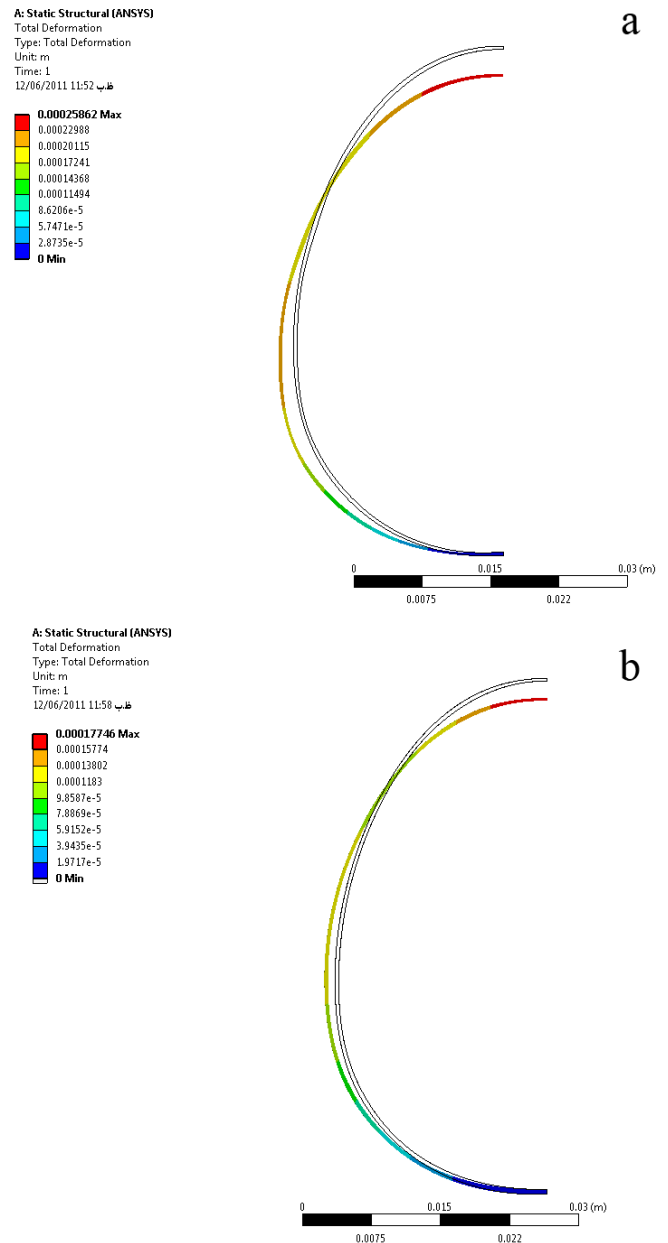
Fig. 6 Models of the hen's egg under point loading (a) With constant thickness (b) with variable thickness
