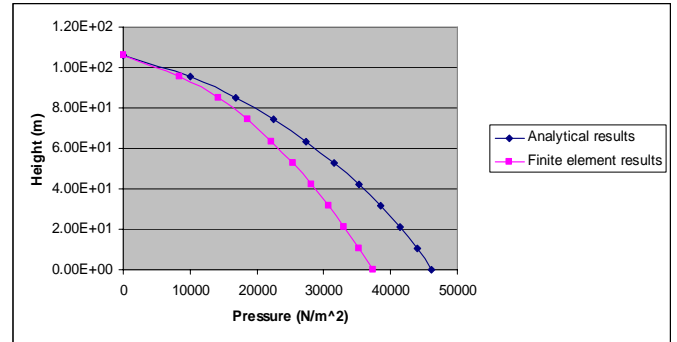
Fig. 7 Hydrodynamic pressure distribution curve by height for dams with L/H = 1
