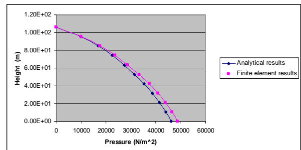
Fig. 9 Hydrodynamic pressure distribution curve by height for dams with L/H = 1
