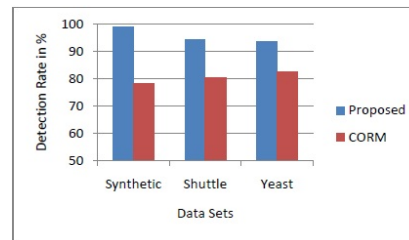
Fig. 2. Outlier Detection Rate
