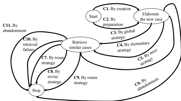
Fig. 4 The retrieval MAP
