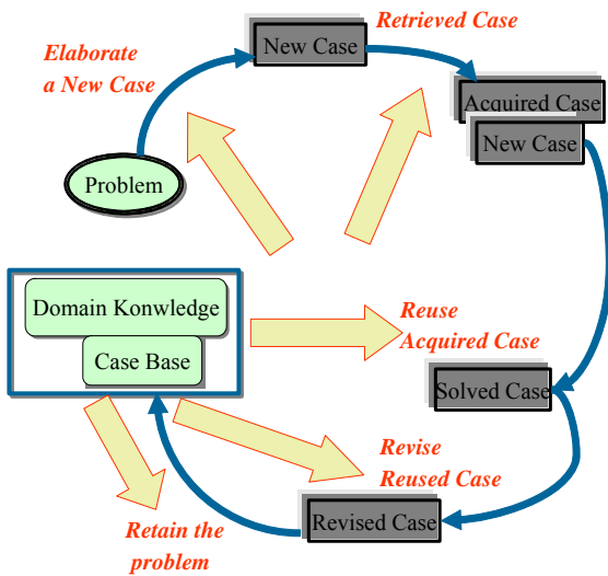
Fig. 1 The CBR reasoning in the SAFRS system
