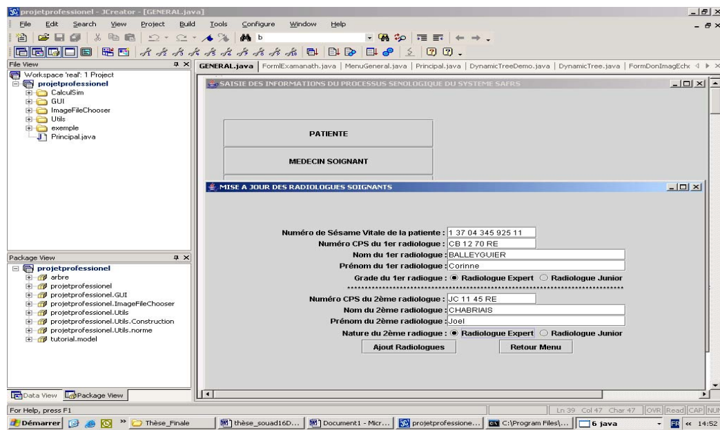
Fig. 8 Dialog box for the 'case author' identification
