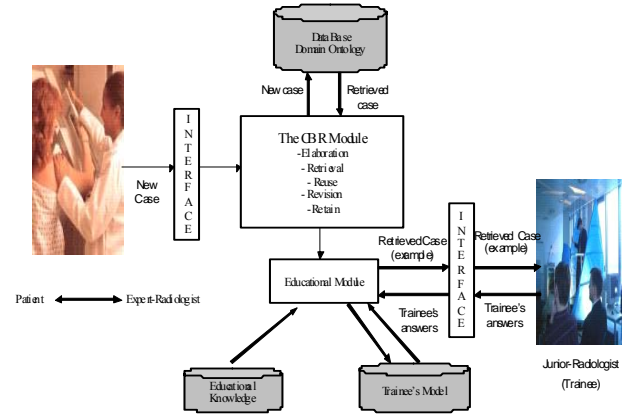
Fig. 2 Architecture of the SAFRS system
