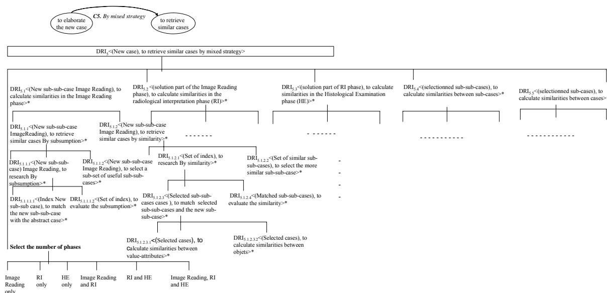
Fig. 7 The mixed strategy (a plan directive: hierarchy of plan contexts)
