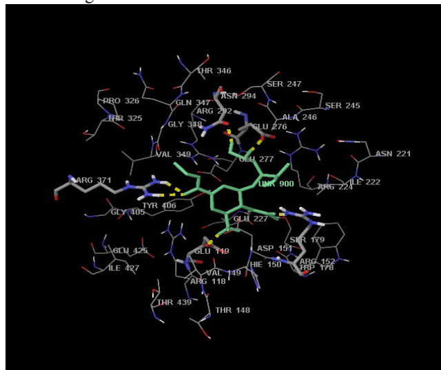
Fig. 2 Snapshot showing the docked position of Oseltamivir analog adiasvssn 10 with N2. The yellow dashed lines are the Hydrogen bonds between the protein and the drug
