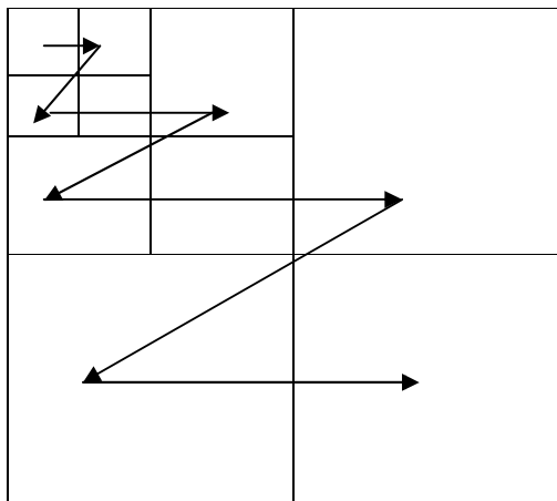
Fig. 2 EZW sub-band structure scanning order
