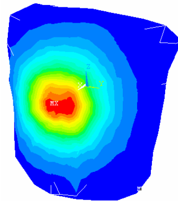
Fig. 12 Magnetic flux density distribution
