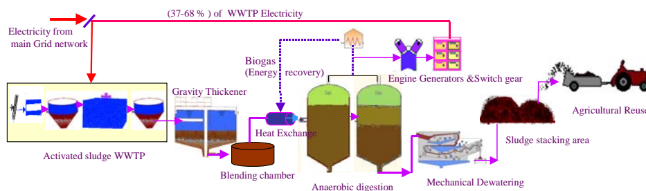
Fig. 2 Flow diagram of the sludge treatment scenario by using anaerobic digestion technology
