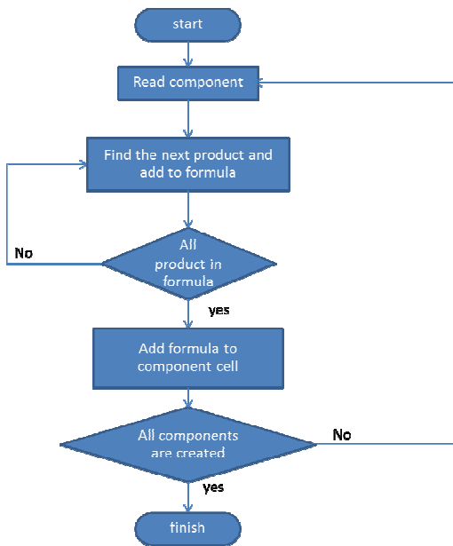
Fig. 3 The flow chart of algorithm
