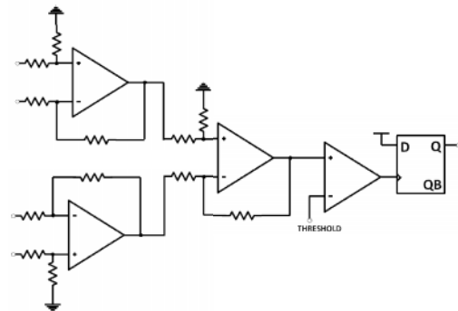
Fig. 5 Sense Resistors' Amplifier
