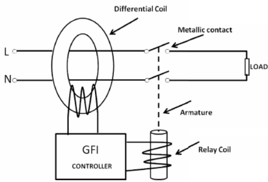
Fig. 3 Ground Fault Isolator
