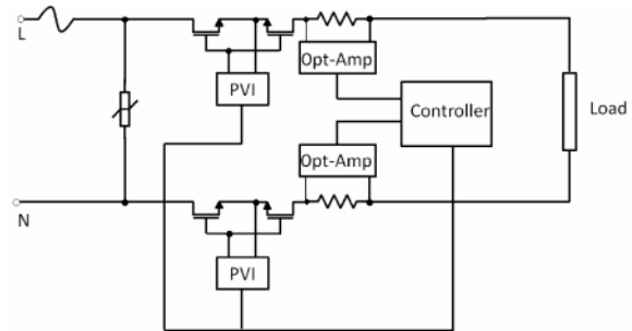
Fig. 4 GFI with Sense Resistors
