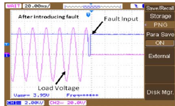
Fig. 8 Voltage after fault induction
