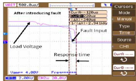
Fig. 9 GFI's response time
