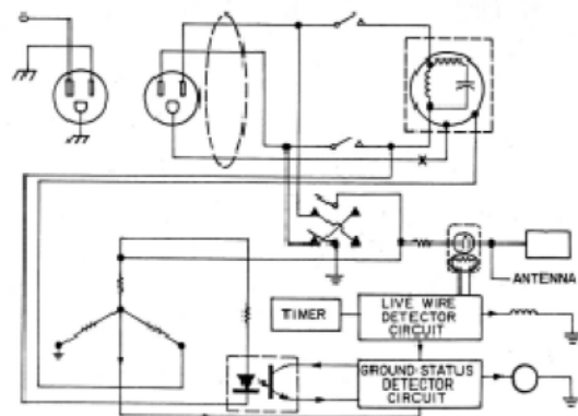
Fig. 2 Grounding Detector
