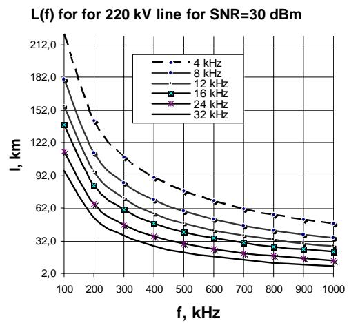
Fig. 8 l(f) for 220 kV line for SNR=30 dBm
