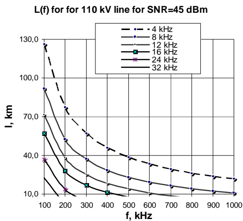
Fig. 5 l(f) for 110 kV line for SNR=45 dBm
