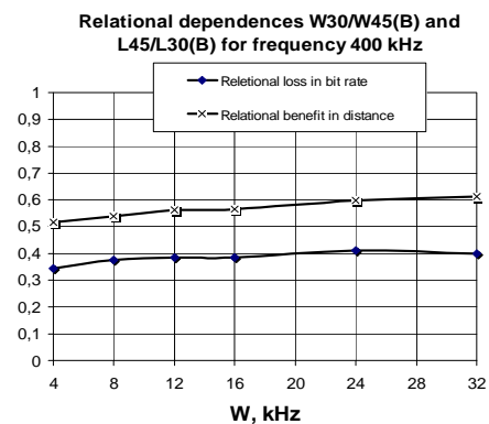
Fig. 9 Relational change of W and L for SNR 45 and 30 dBm
