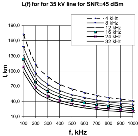
Fig. 4 l(f) for 35 kV line for SNR=45 dBm
