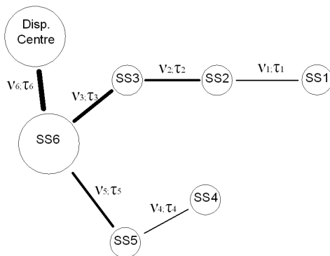
Fig. 10 Model of the network with pPLC links
