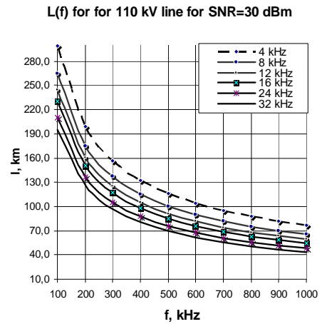
Fig. 7 l(f) for 110 kV line for SNR=30 dBm
