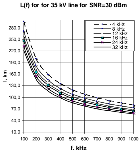
Fig. 6 l(f) for 35 kV line for SNR=30 dBm
