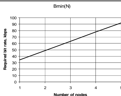
Fig. 13 Dependence between minimal required bit rate and number of nodes in multi-segment link
