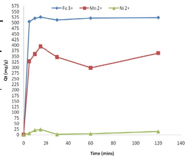
Fig. 8 Metal uptake capacity of Desmodemus sp.
