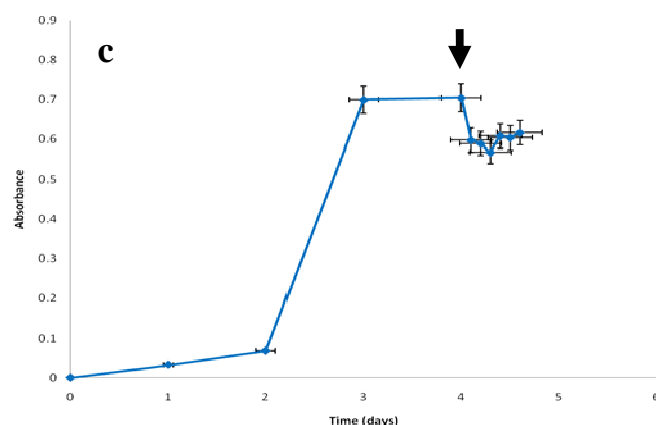
Fig. 9 Effect of (a) Nickel, (b) Manganese and (c) Iron, on growth rate of algae cells.
