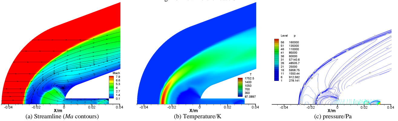
Fig. 11 Flow field of case 4
