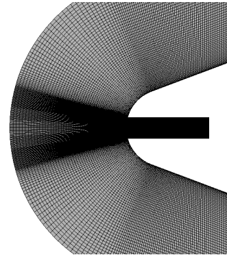
Fig. 2 Symmetry plane grid ( L=32\text{mm} , D=8\text{mm} )
