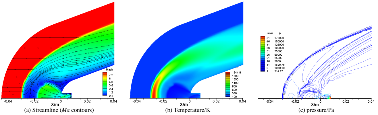
Fig. 8 Flow field of case 1
