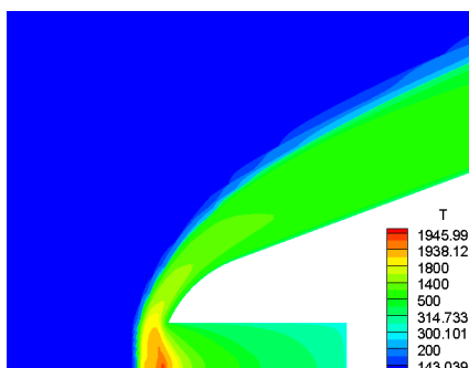
Fig. 7 Temperature/K contours of nose-tip with D=12\text{mm} cavity
