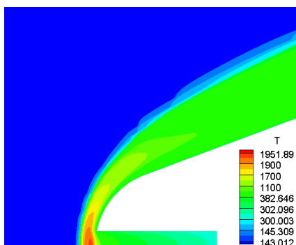
Fig. 6 Temperature/K contours of nose-tip with D=6\text{mm} cavity
