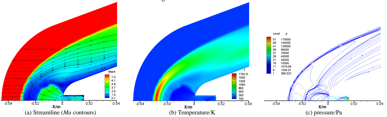
Fig. 9 Flow field of case 2
