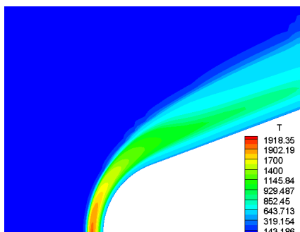
Fig. 5 Temperature/K contours of blunt cone
