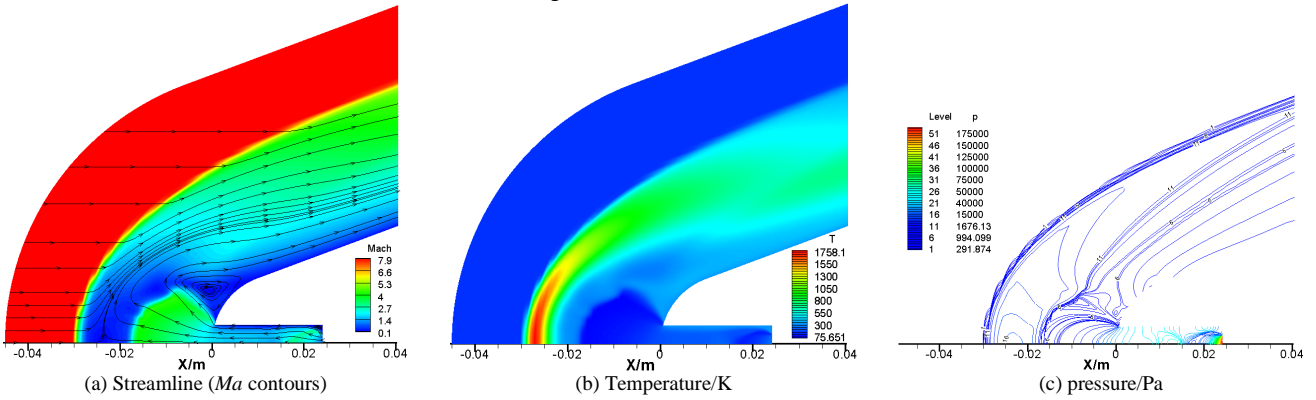
Fig. 10 Flow field of case 3
