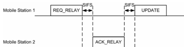
Fig. 4 Messages REQ_RELAY, ACK_RELAY, and UPDATE
