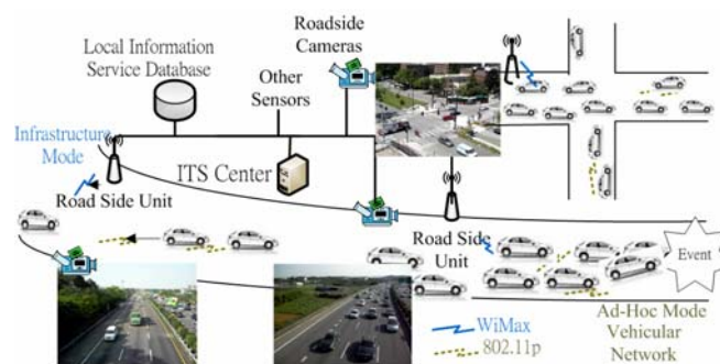
Fig. 1 System framework
