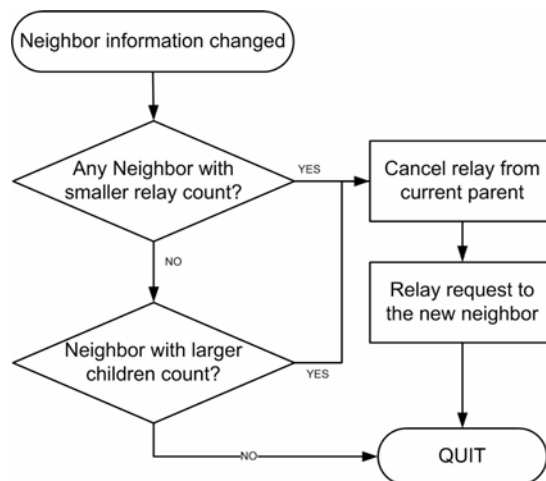
Fig. 6 Relay improvement procedure
