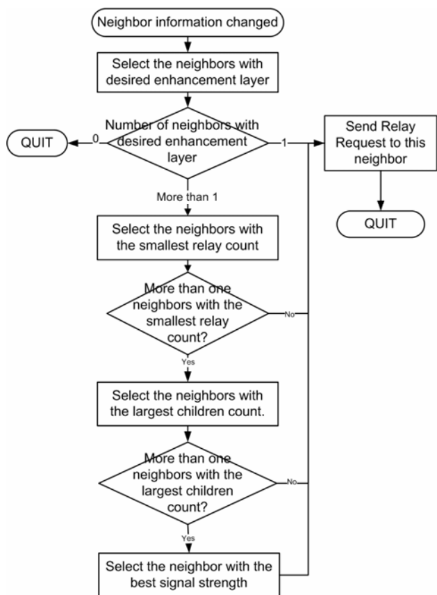
Fig. 5 Relay check procedure
