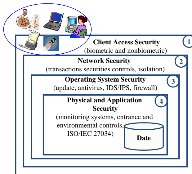
Fig. 1 Data security levels
