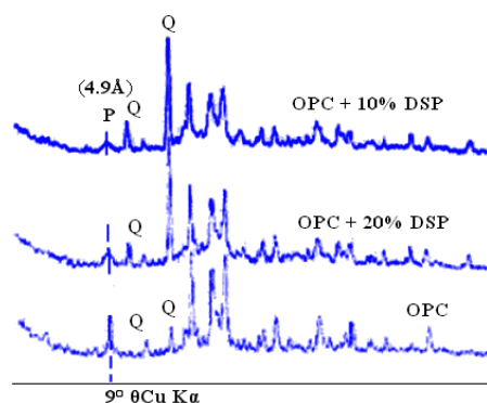
Fig. 6 X Diffractograms of cement pastes in the presence of DSP in 14 days
