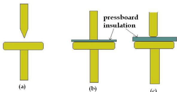
Fig. 3 Schematic diagram of electrode systems employed (a) point-plane electrode (b) rod-plane electrode with insulation. (c) plane-plane electrode with insulation.
