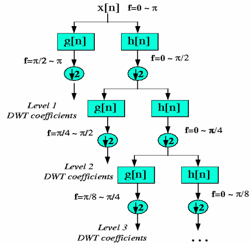
Fig. 5 Wavelet decomposition tree
