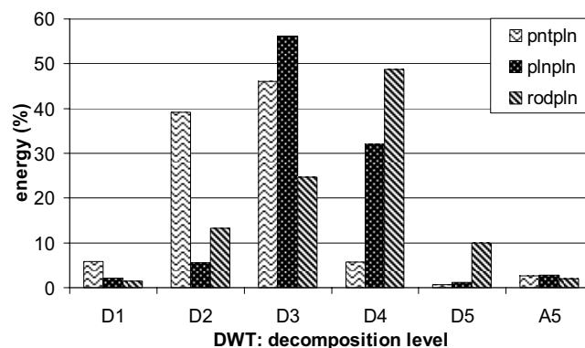
Fig. 11 Energy distribution of PDAE signal for different electrode system
