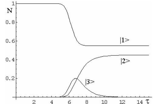
Fig. 4 The temporal dynamics of the populations of nuclear levels |1\rangle , |2\rangle and |3\rangle . The time is normalized on \tau_3 , here \tau_p = 1 , G = 0.5 , \tau_0 / \tau_p = 6
