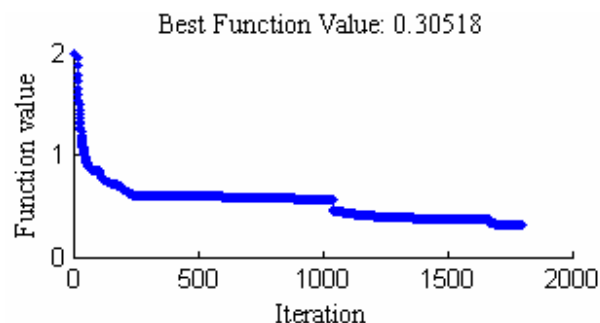
Fig.7.b Best fitness curve of GA-GPS
