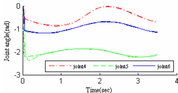
Fig. 9.d Joint Desired and actual joint angles of circular trajectory for unfiltered PID with disturbance
