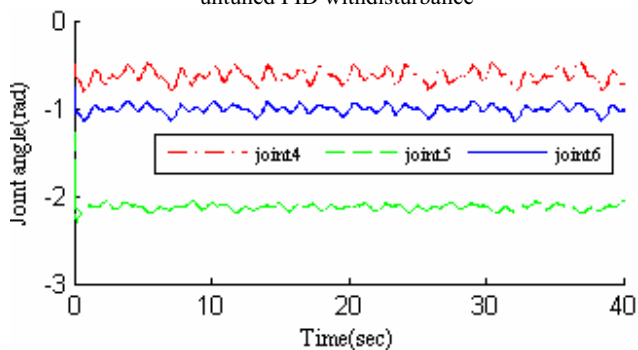
Fig. 10.d Desired and actual joint angles of butterfly trajectory for unfiltered PID with disturbance
