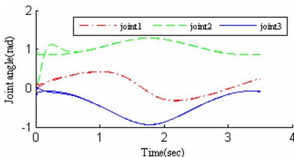
Fig. 9.c Joint Desired and actual joint angles of circular trajectory for unfiltered PID with disturbance
