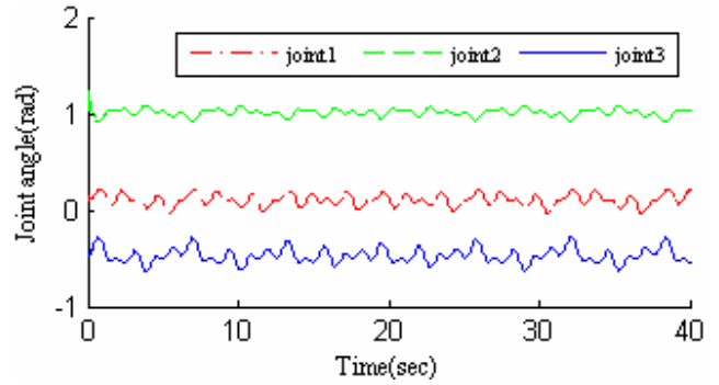
Fig. 12.a Desired and actual joint angles of butterfly trajectory for GA-GPS tuned PID without disturbance
