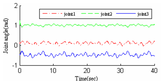
Fig. 12.c Desired and actual joint angles of butterfly trajectory for GA-GPS tuned PID with disturbance
