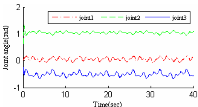
Fig. 10.c Desired and actual joint angles of butterfly trajectory for unfiltered PID with disturbance
