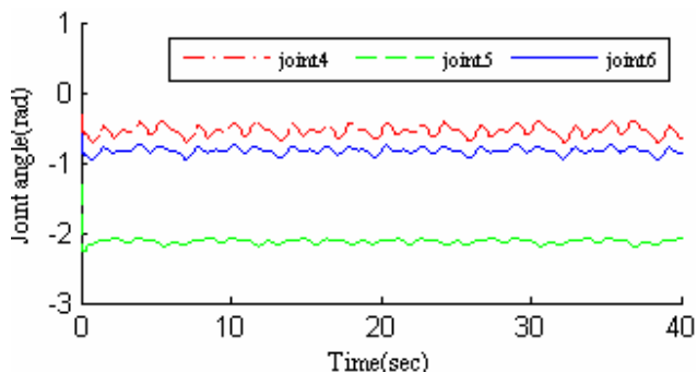
Fig. 10.b Joint Desired and actual joint angles of butterfly trajectory for unfiltered PID without disturbance
