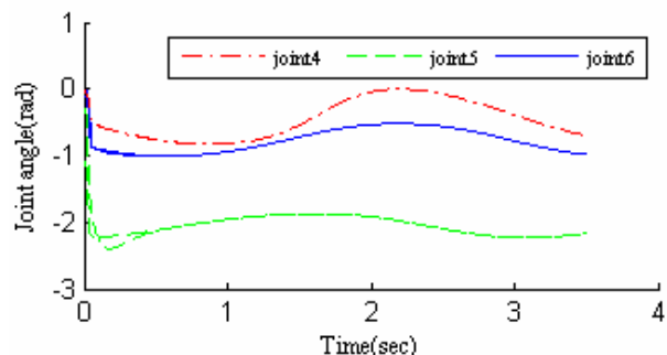
Fig. 9.b Desired and actual joint angles of circular trajectory for unfiltered PID without disturbance
