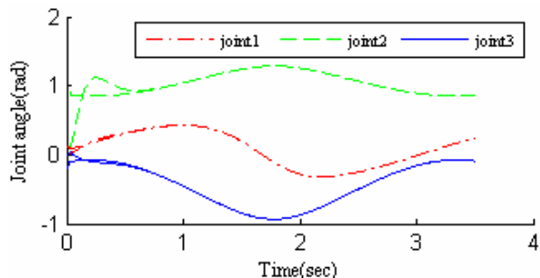
Fig. 9.a Desired and actual joint angles of circular trajectory for unfiltered PID without disturbance
