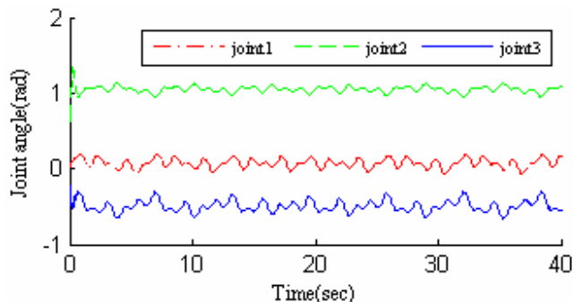
Fig. 10.a Desired and actual joint angles of butterfly trajectory for unfiltered PID without disturbance
