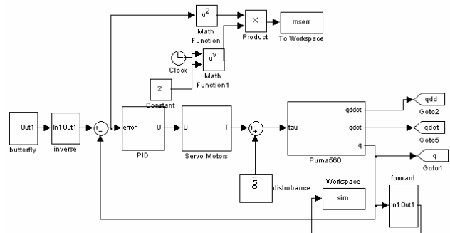
Fig. 3 Simulink diagram of PUMA560 system
