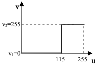
Fig. 2 Thresholding transformation curve [1].
