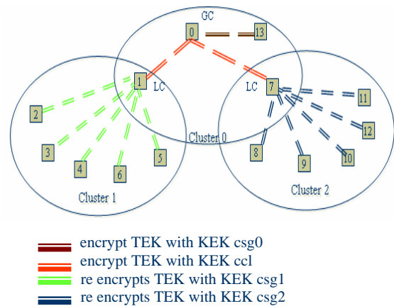
Fig. 3 Multicast key distributions
