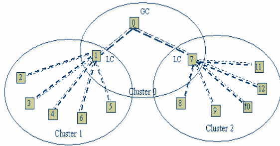
Fig. 2 Enhanced OMCT with DSDV
