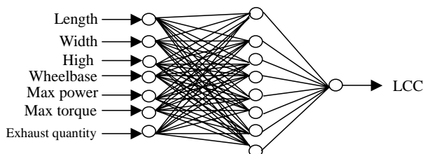
Fig. 3 Structure of BP ANN
