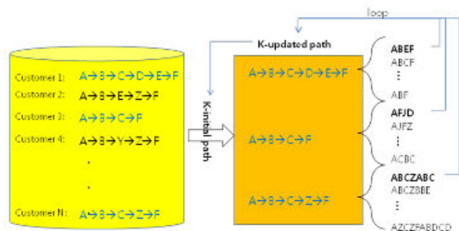
Fig. 8 Procedure of suggested method
