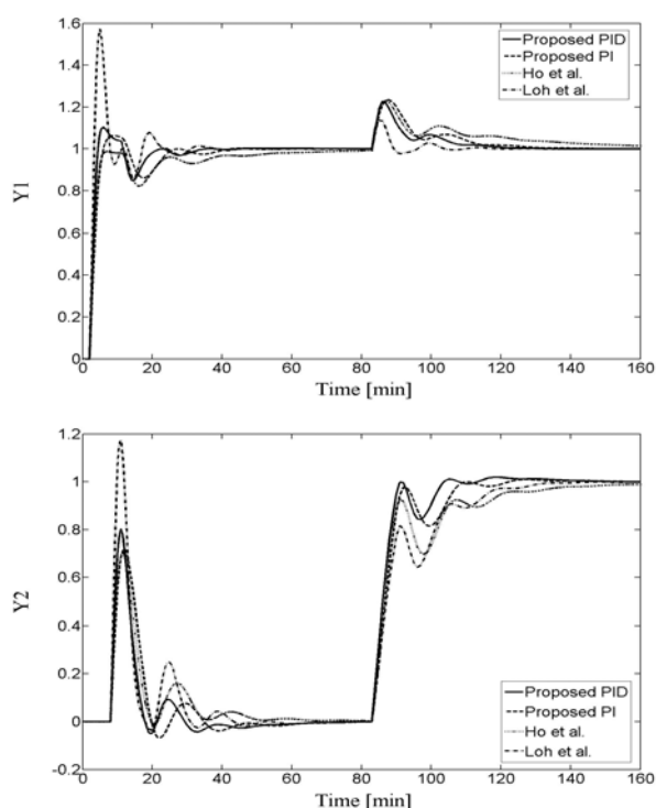
Fig. 3 Closed-loop time responses for WB column.
