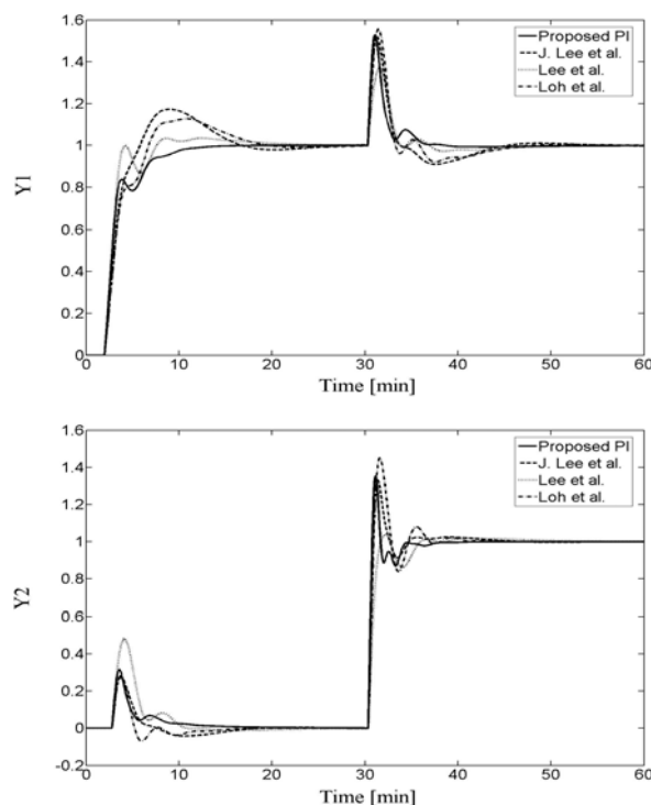
Fig. 4 Closed-loop time responses for VL column.
