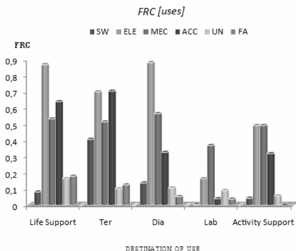
Fig. 5 Number of Failures per Category per n° of devices classified according to the "destination of use" classification
