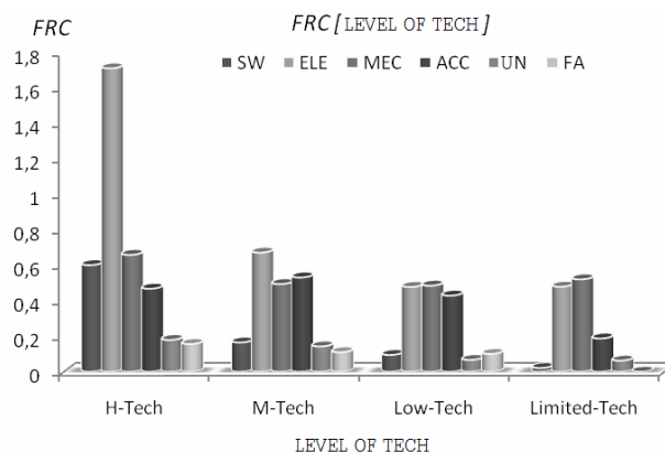
Fig. 4 Number of Failures per Category per n° of devices classified according to the technological complexity classification
