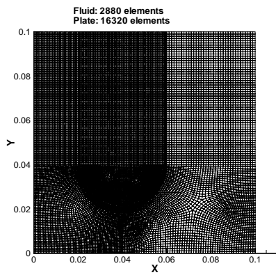
Fig. 8: Mesh used for the U-shaped channel problem
