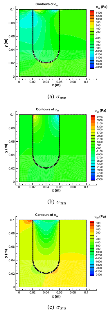
Fig. 13: Stress contours for the U-shaped channel problem
