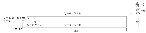
Fig. 2: Computational domain for flow over a backward facing step
