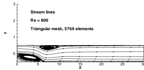
Fig. 3: Streamlines for flow over a backward facing step
