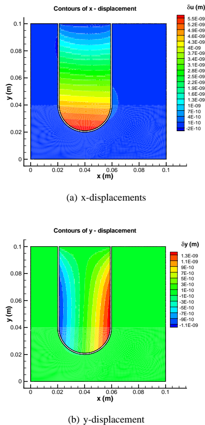
Fig. 12: Displacement contours for the U-shaped channel problem
