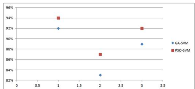
Fig. 9 Optimal Classifier Analysis
