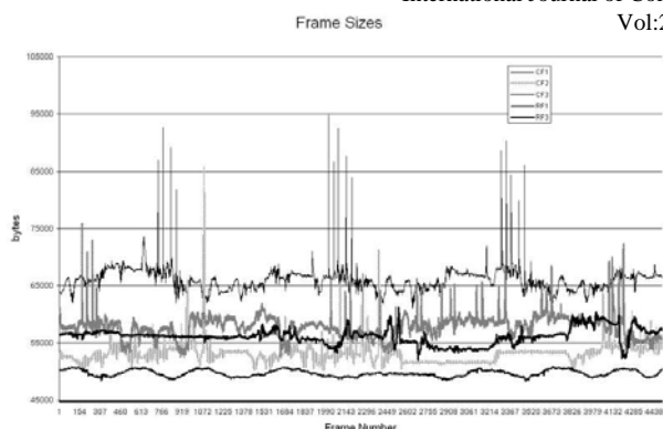
Fig. 5. Size evolution of streams with q=80
