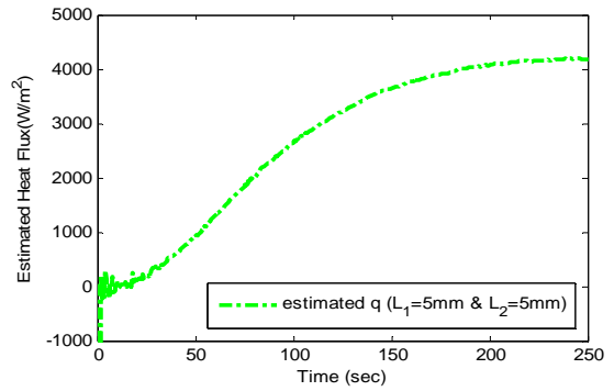
Fig. 4d The estimated heat flux ( L = 9mm )
