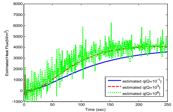
Fig. 6a The estimation results of the heat flux. ( Q = 10^{-1}, 10^3 , and 10^6 )
