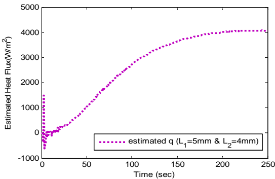
Fig. 4c The estimated heat flux ( L = 10mm )
