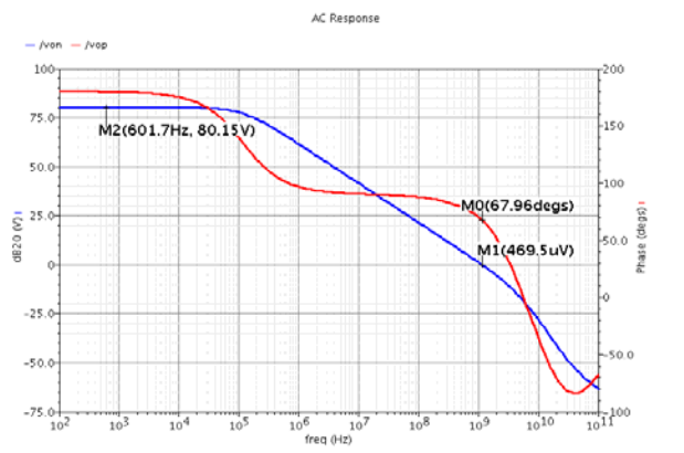
Fig. 6 AC response
