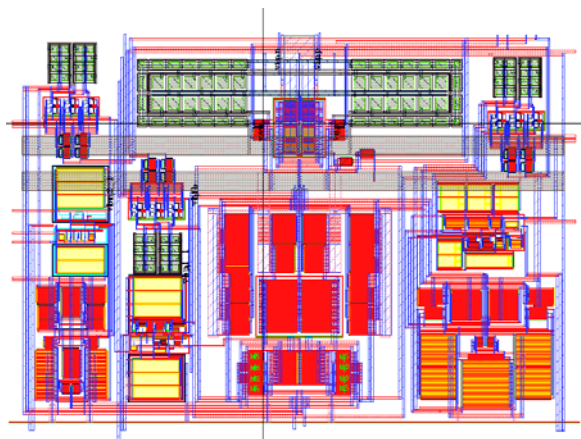
Fig. 5 The whole Layout
