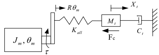
Fig. 6 Free-body diagram of the feed drive system.
