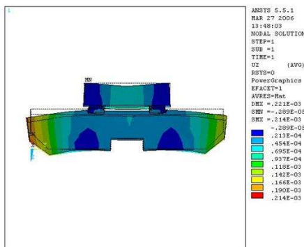
(a) Static displacement by gravity
