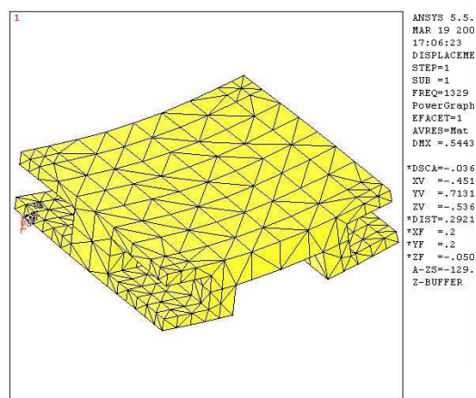
(c) Shape optimization for the table
