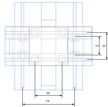
Fig. 5 System assembles of main mechanical structures for a feed drive system.
