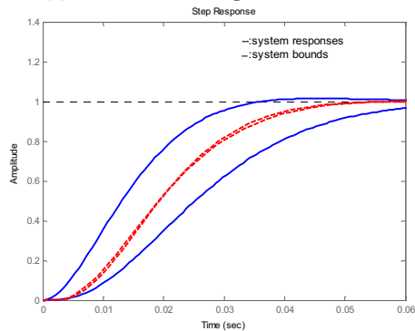
(b) Time domain response of Y axis
