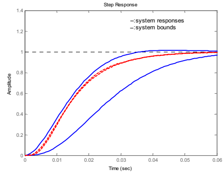
(a) Time domain response of X axis
