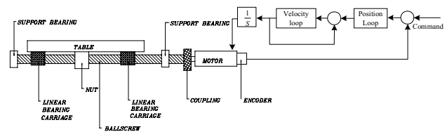
Fig. 3 Typical mechatronic feed drive system
