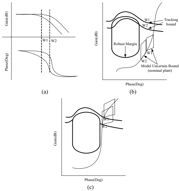
Fig. 7 QFT design procedures.
