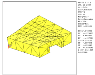
(c) Table (mass: 60 Kg, natural frequency: 1323Hz)
