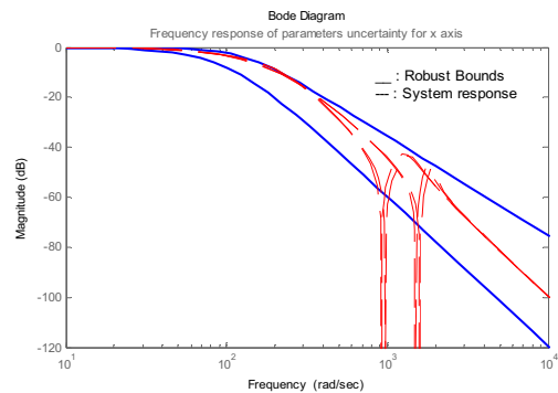
(c) Frequency responses of X axis
