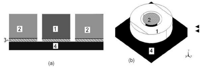
Fig. 2 The schematic diagram the tactile sensor showing a) the cross sectional and b) the three
