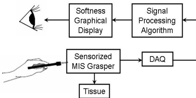
Fig. 1 The schematic diagram of the complete system
