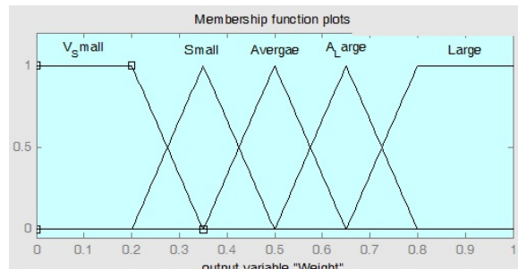
Fig. 6 The output membership function
