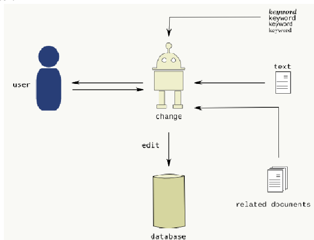
Fig. 3 The Data collector & editing agent
