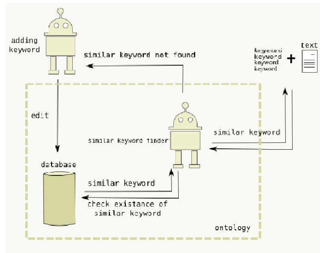
Fig. 2 The Keyword agent
