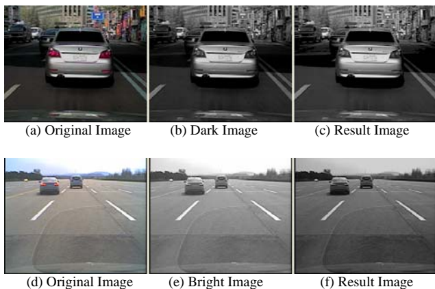
Fig. 2 Auto intensity control considering the image brightness
