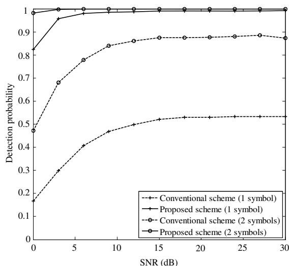
Fig. 4. Detection probabilities of the conventional and the proposed schemes when the timing synchronization error is 80 samples.
