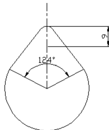
Fig. 8 Modified intake cam
