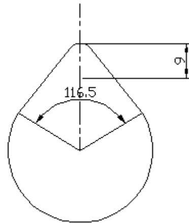
Fig. 7 Conventional intake cam
