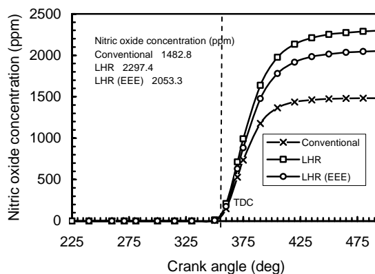
Fig. 19 Comparison of Nitric oxide concentration for Conventional, LHR and LHR (EEE) for the diesel fuel supplied (0.0694g/cycle/cylinder) at 1500 rpm
