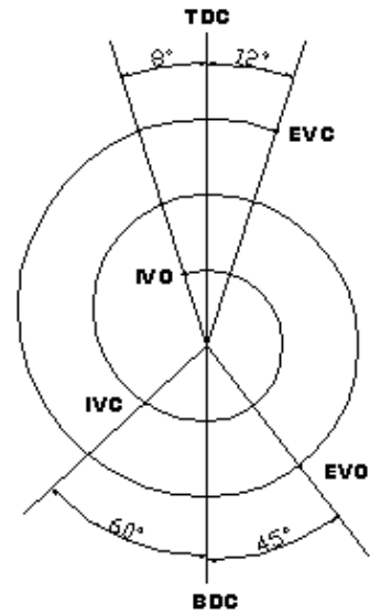
Fig. 6 Extended expansion cycle valve timing diagram
