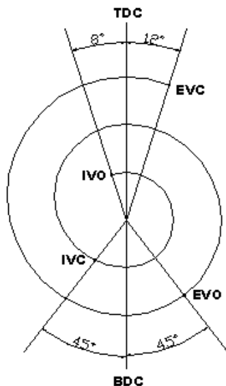
Fig. 5 Conventional valve timing diagram
